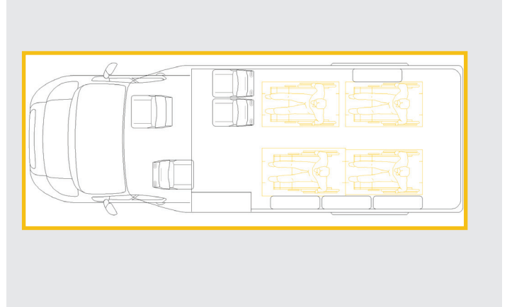
SINGLE REAR AXLE Wheelchair layout
